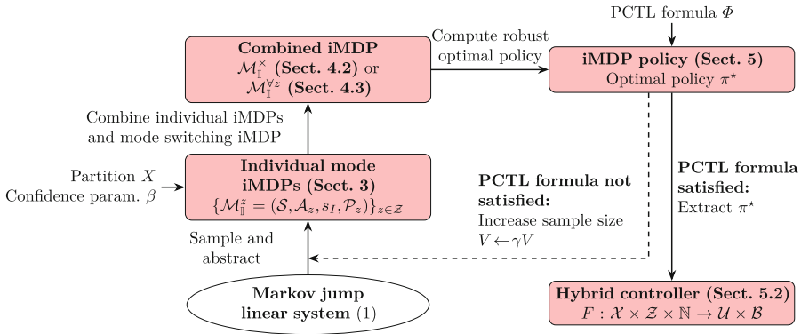
Fig. 1. Approach for synthesising a provably-correct controller for an MJLS.
