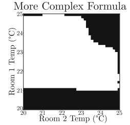
Fig. 6. States that satisfy (in white) the general PCTL formula in (17) (Assumption A).
